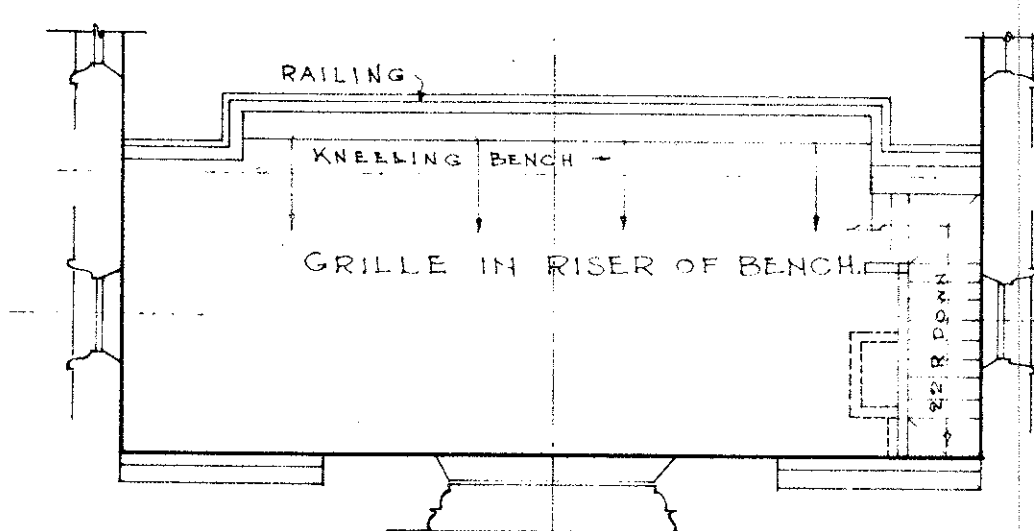
HEATING LAYOUT FOR BALCONY PLAN OF BALCONY
