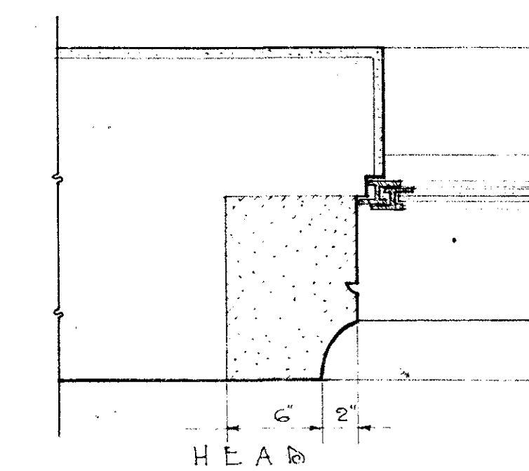
SECTIONS OF TYPICAL CASEMENT WINDOWS SCALE 1 1/2" = 1'-0"
