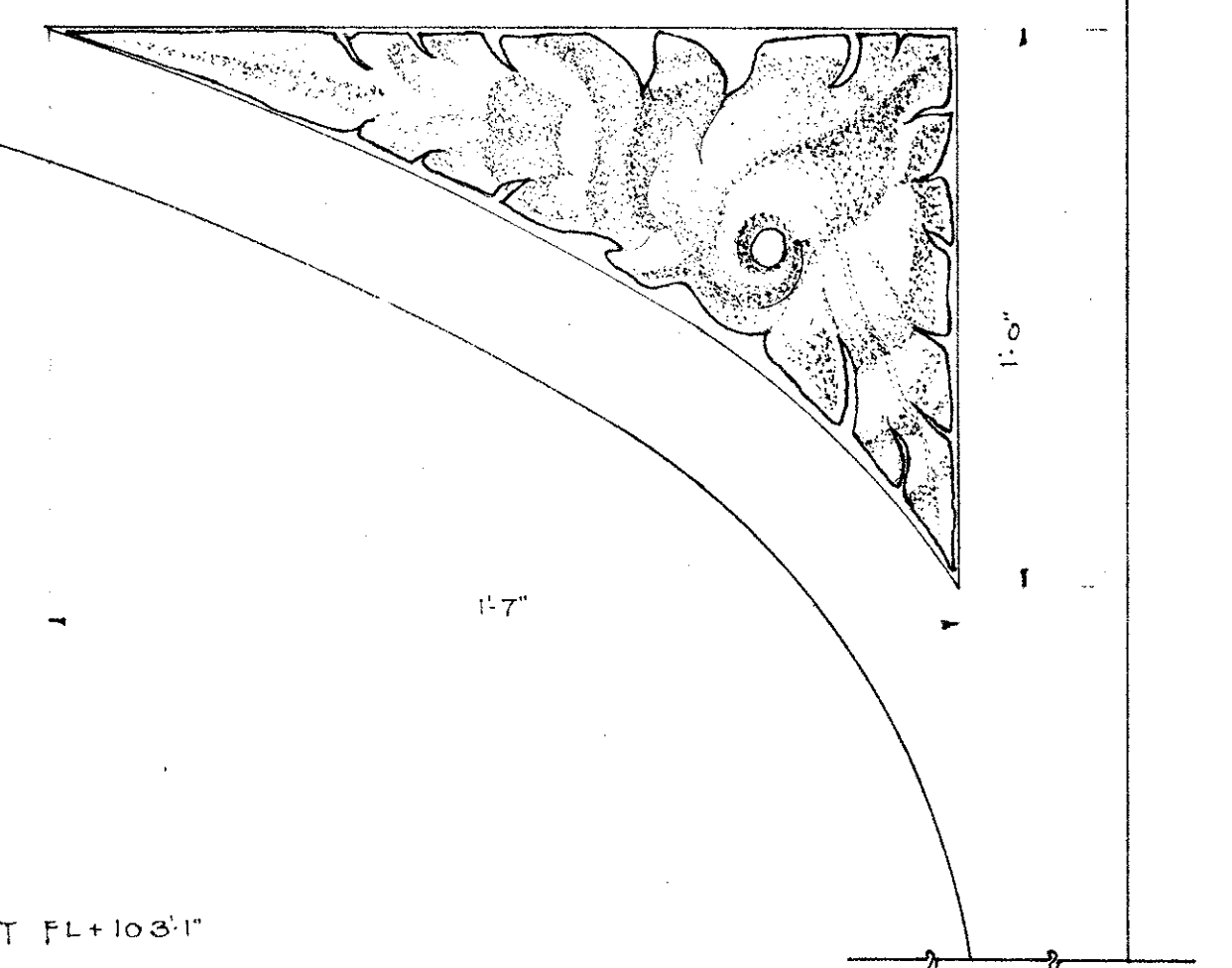
3" DETAIL OF STONE SPANREL
