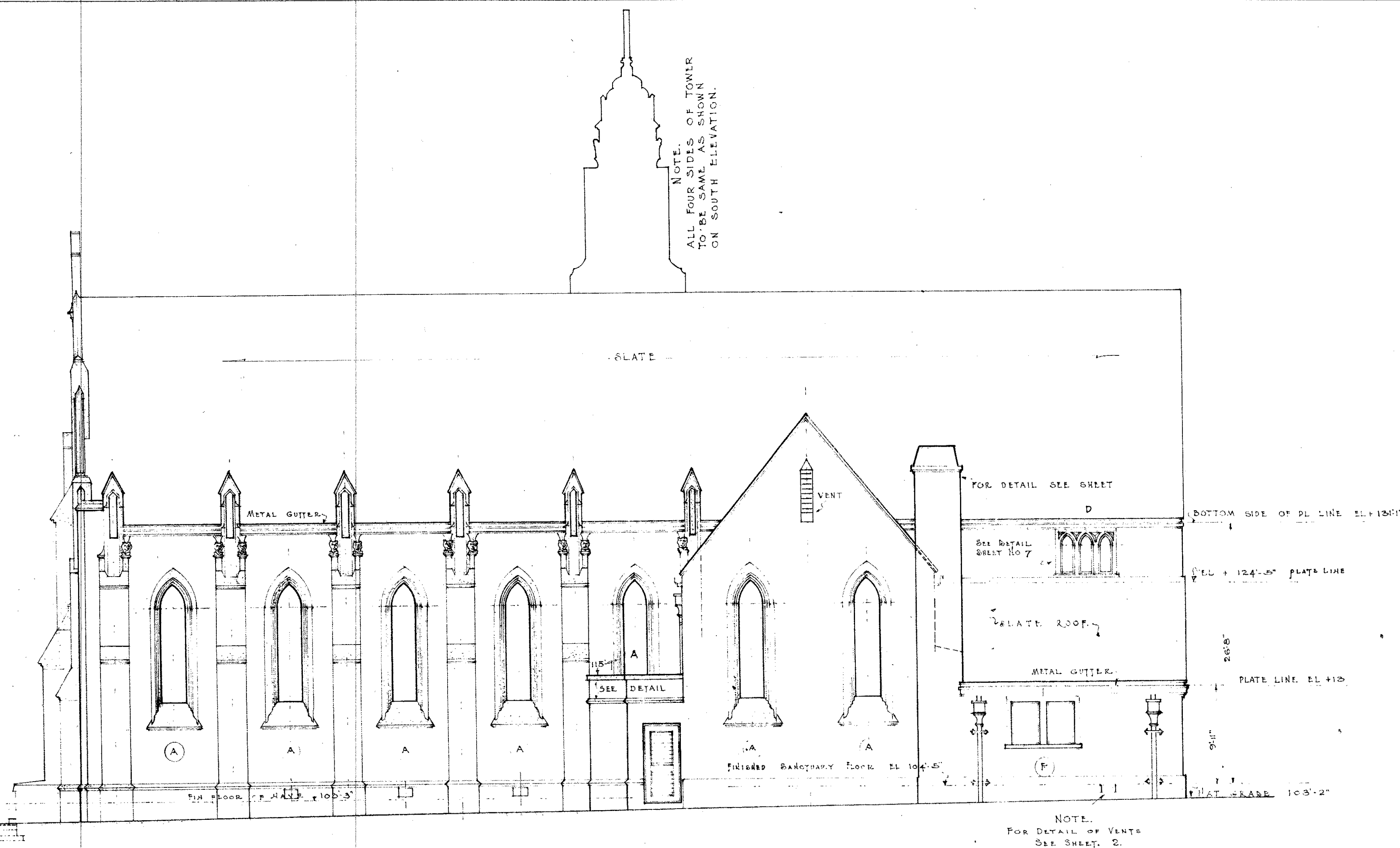
EAST ELEVATION SCALE 1/8"=1'-0"
