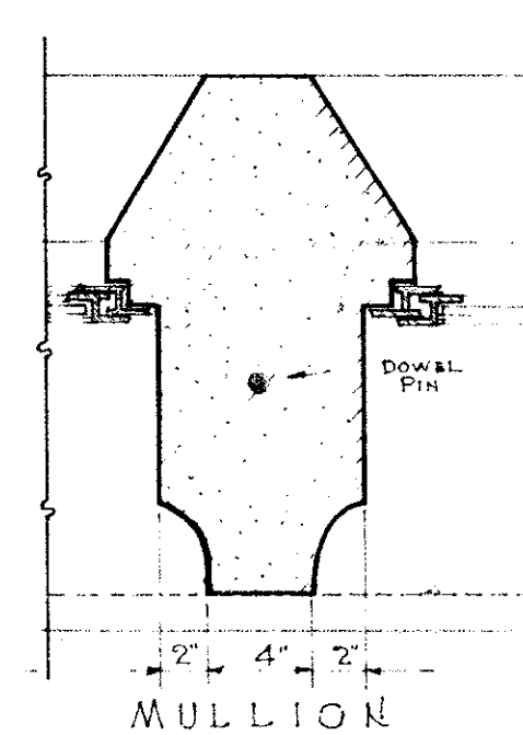
SECTIONS OF TYPICAL CASEMENT WINDOWS SCALE 1 1/2" = 1'-0"
