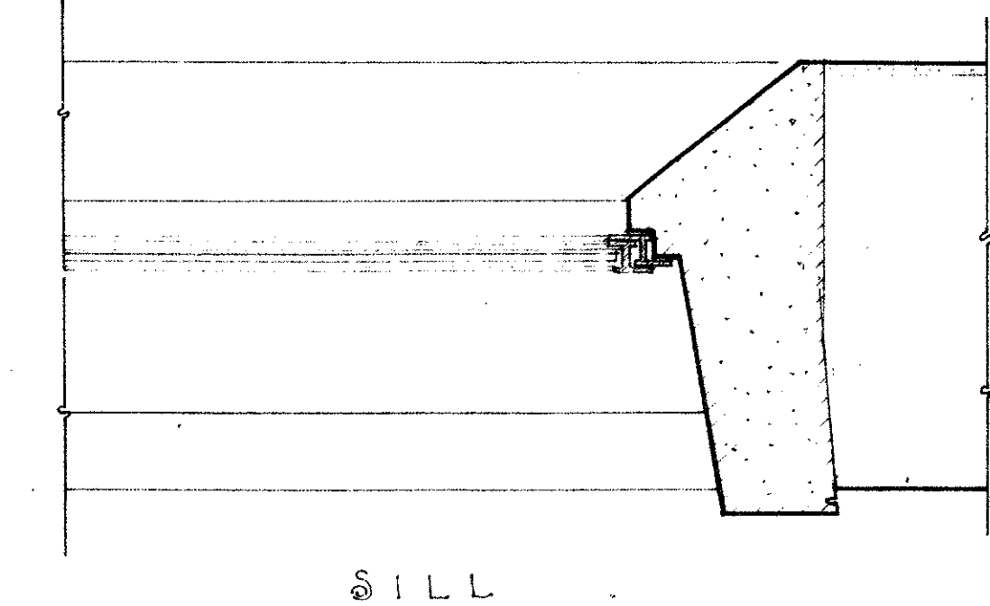
SECTIONS OF TYPICAL CASEMENT WINDOWS SCALE 1 1/2" = 1'-0"
