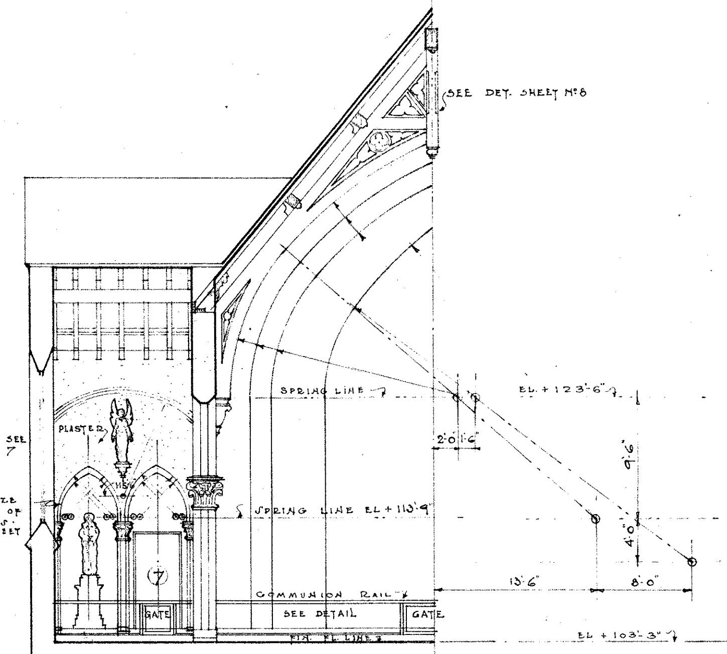
CROSS SECTION S-S
