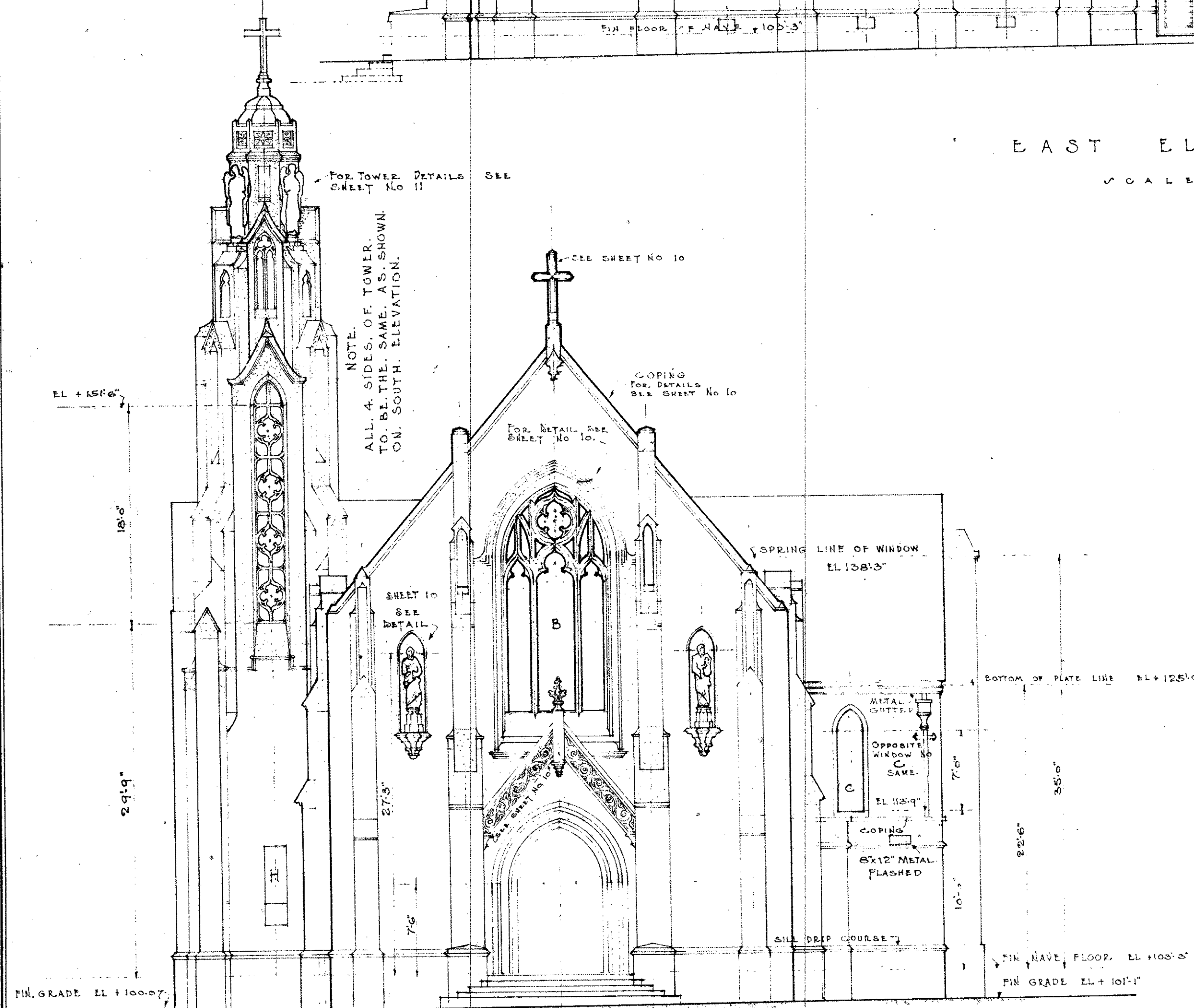
SOUTH ELEVATION SCALE 1/8"=1'-0"
