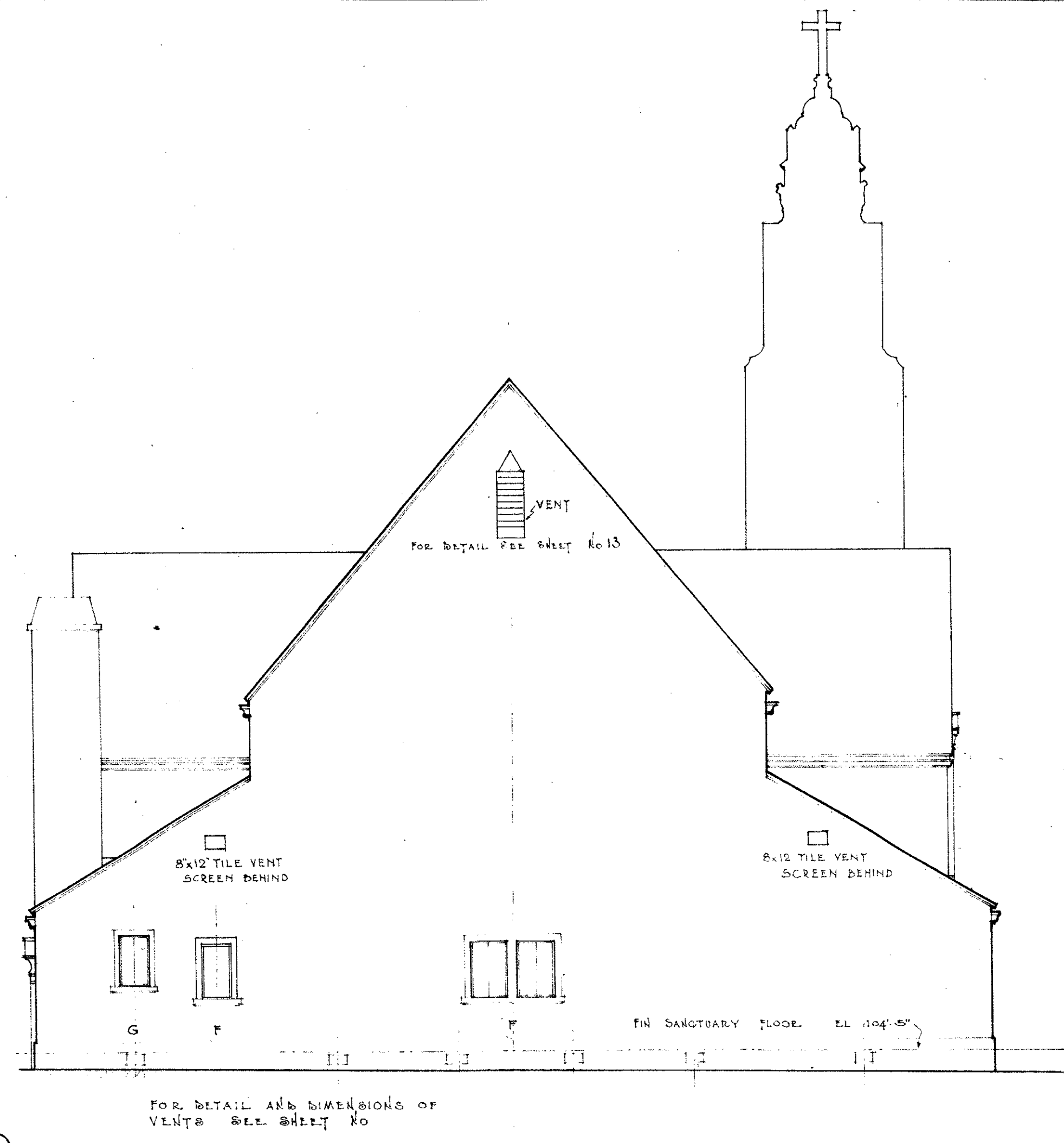
NORTH ELEVATION SCALE 1/8"=1'-0"
