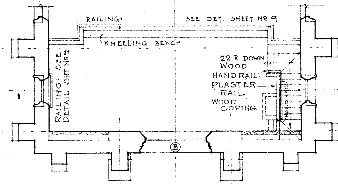
BALCONY FLOOR PLAN
