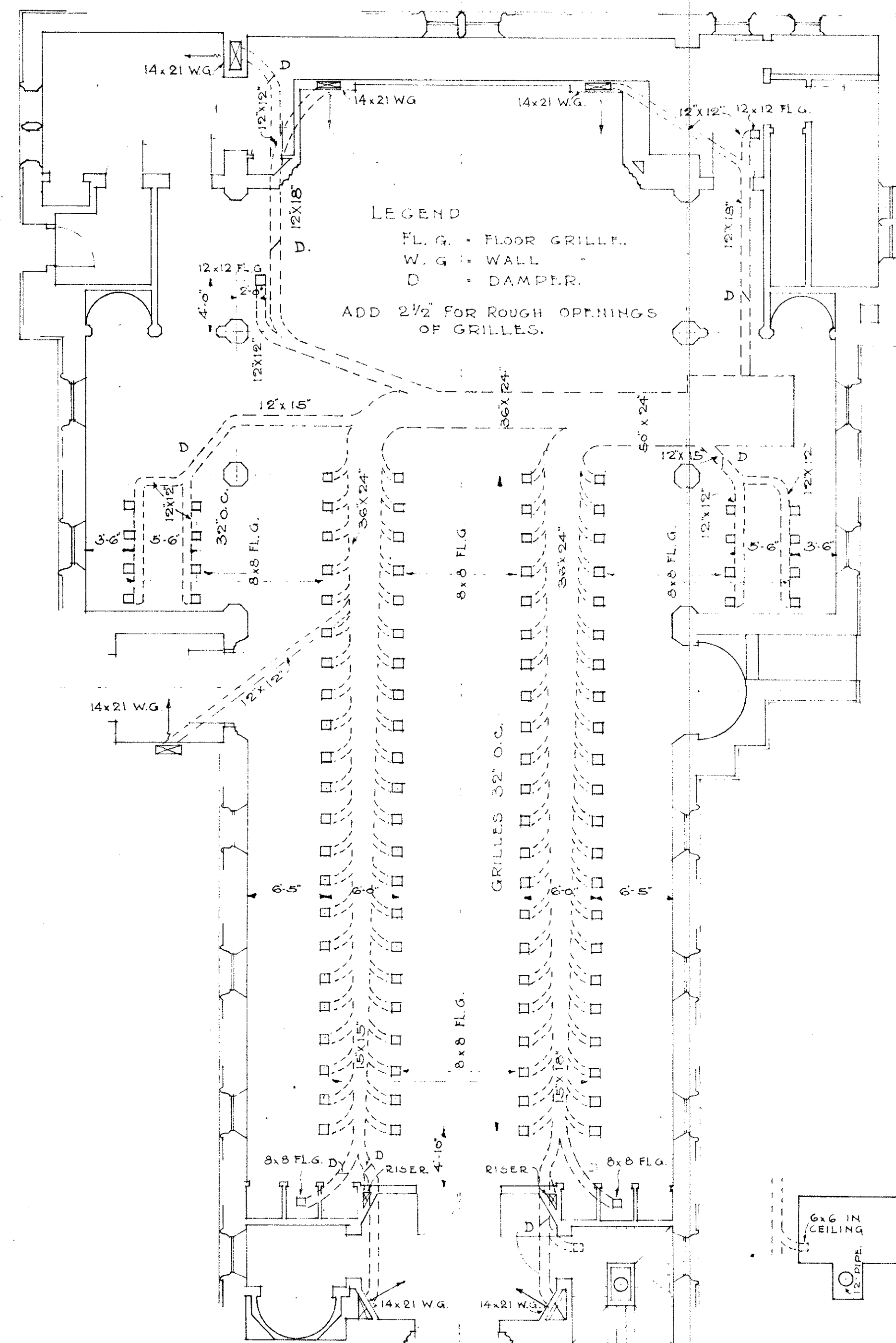
PLAN OF BLOWER ROOM IN BASEMENT.
