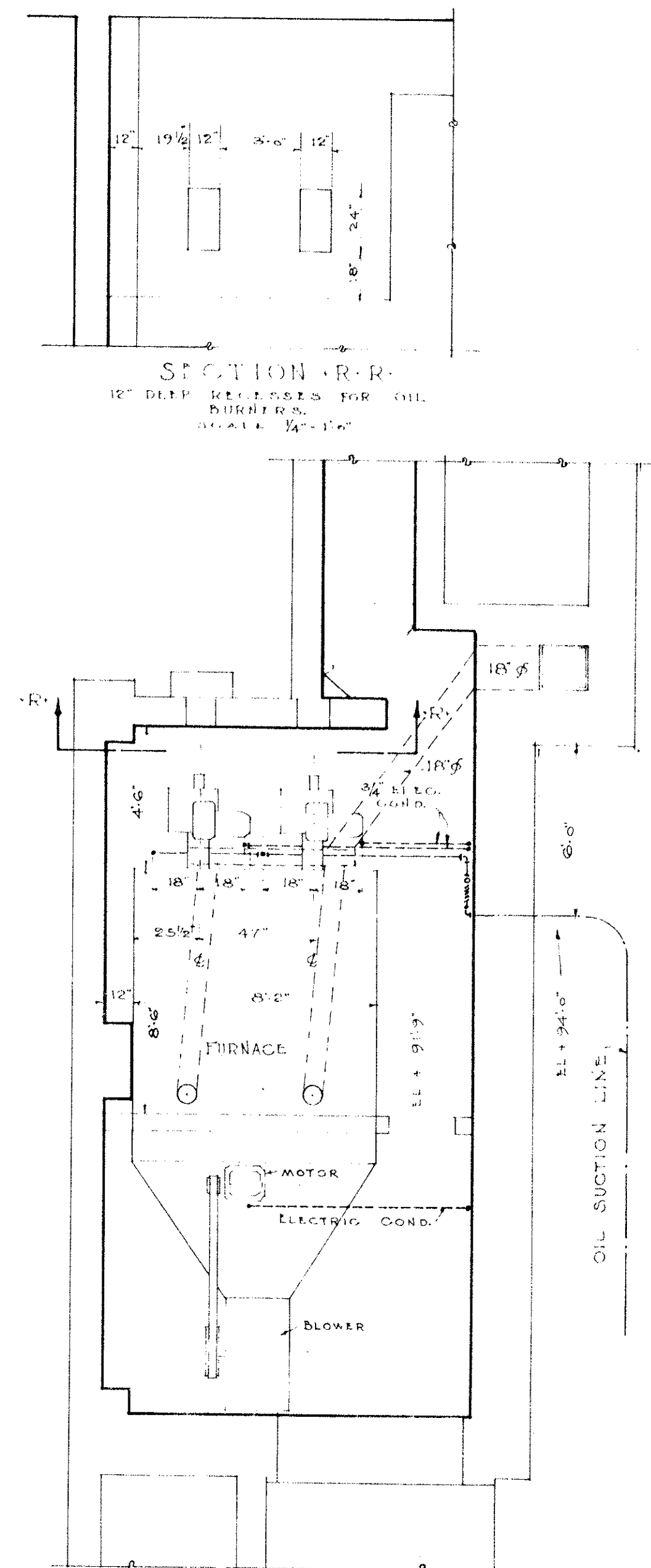
PLAN OF HEATER ROOM SHOWING POSITION OF FURNACE AND FANS. SCALE 1/4\"/>
