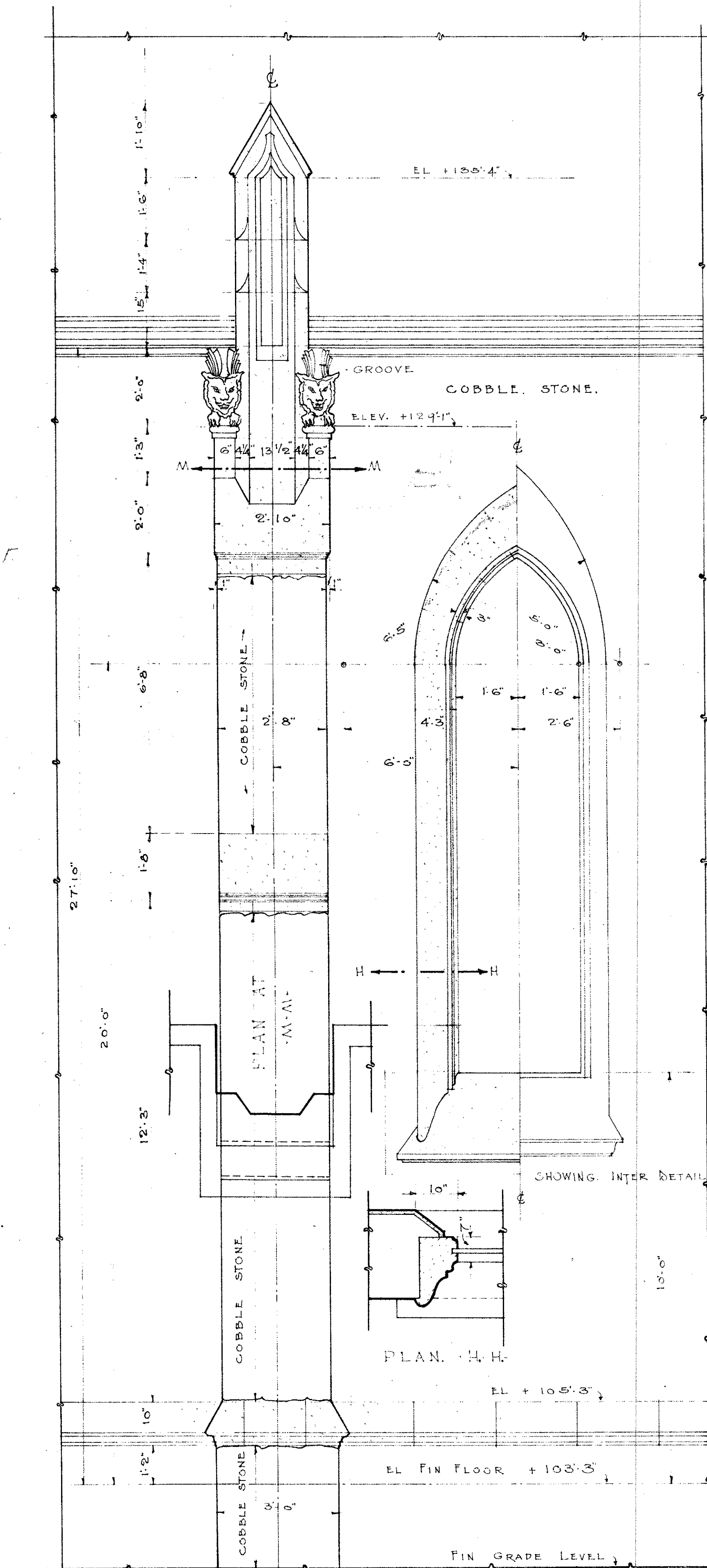
DETAIL OF EXTERIOR WALL BUTTRESS AND WINDOW SCALE 1/2" = 1'-0"
