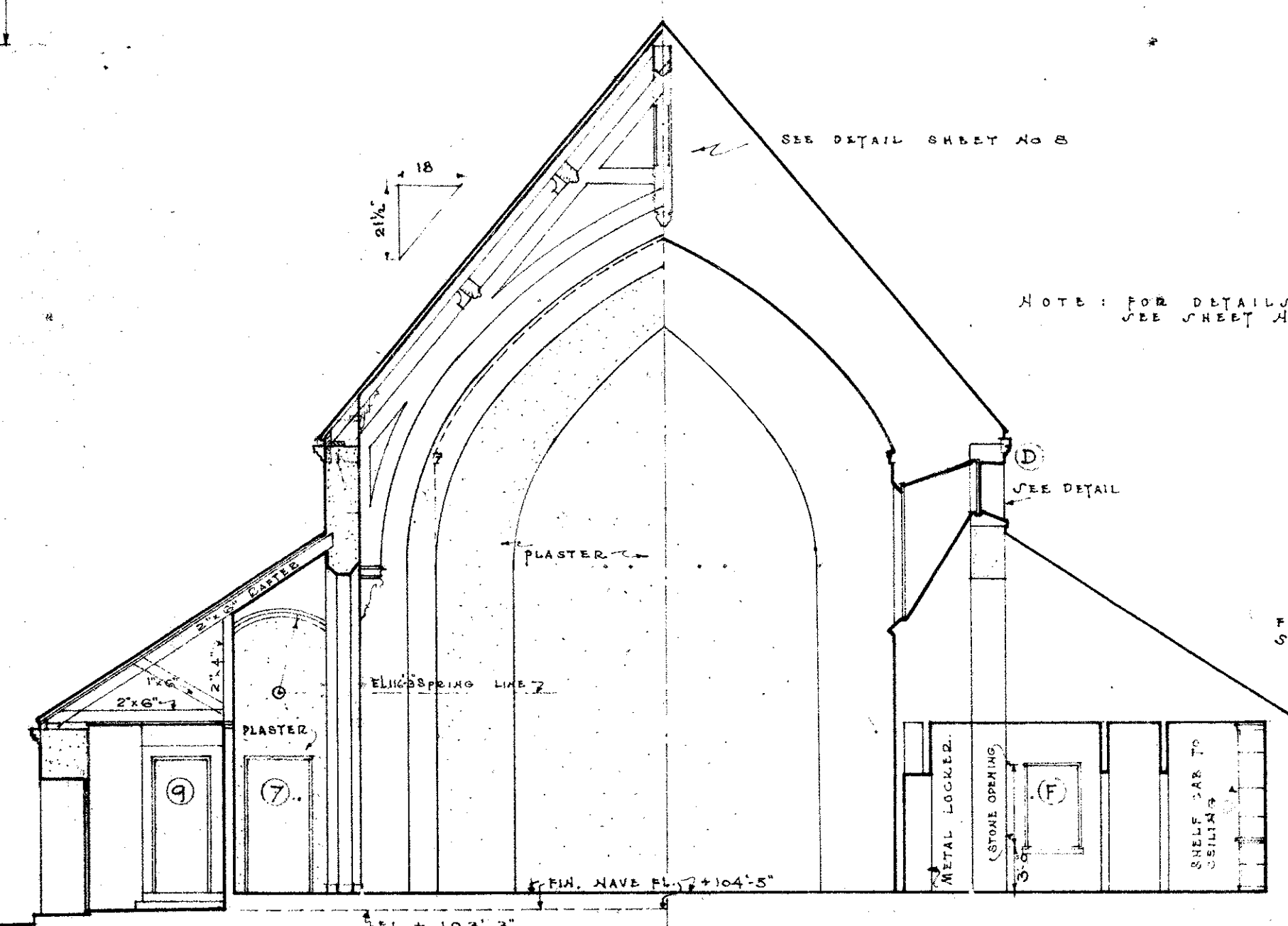
CROSS SECTION R-R
